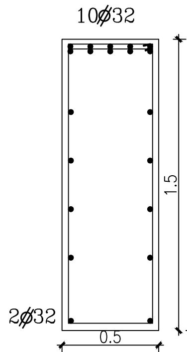
Section 3-3
