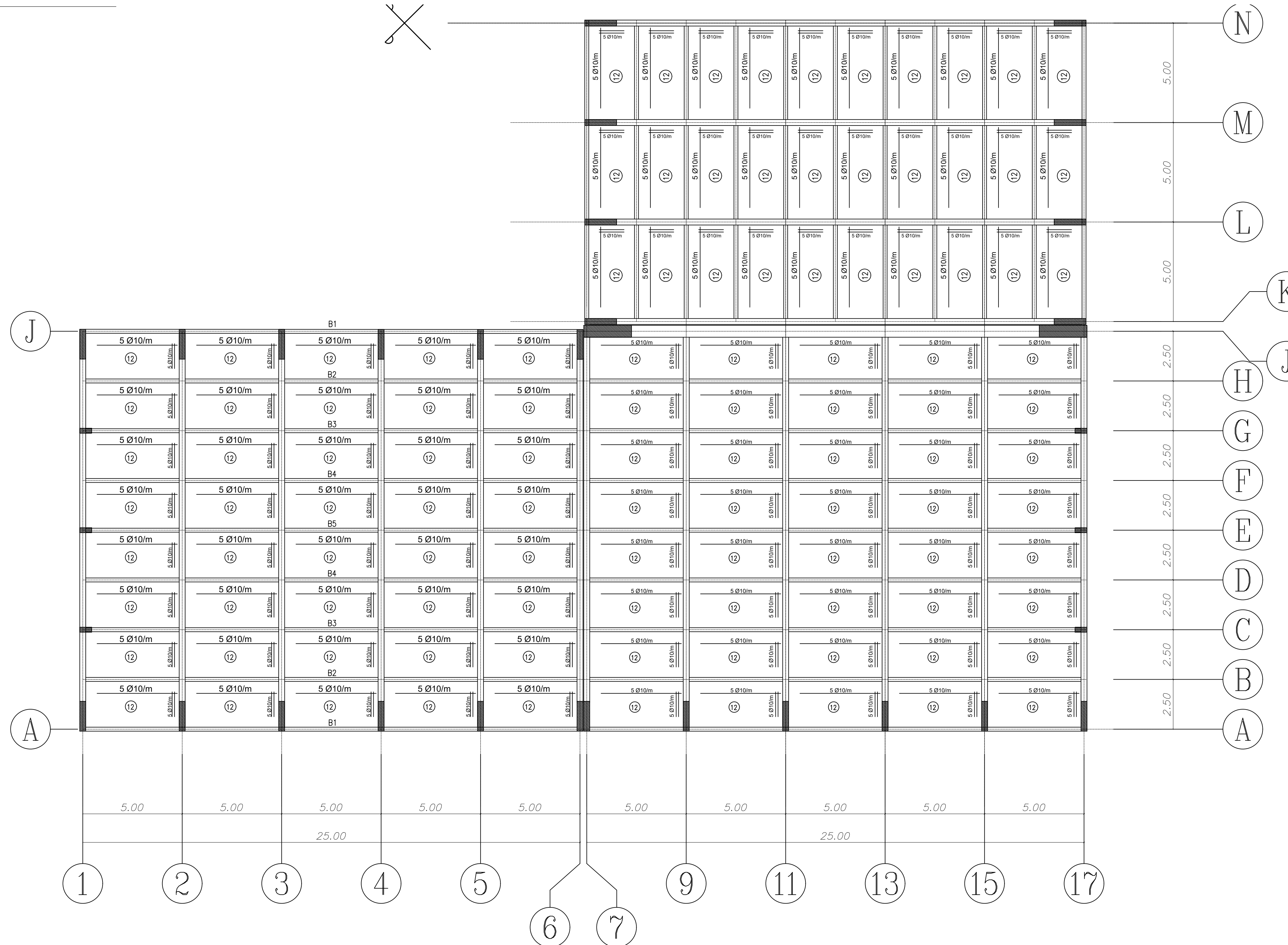
Typical Slab RFT
