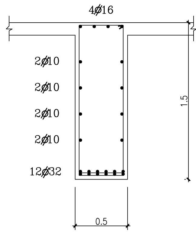
Section 1-1
