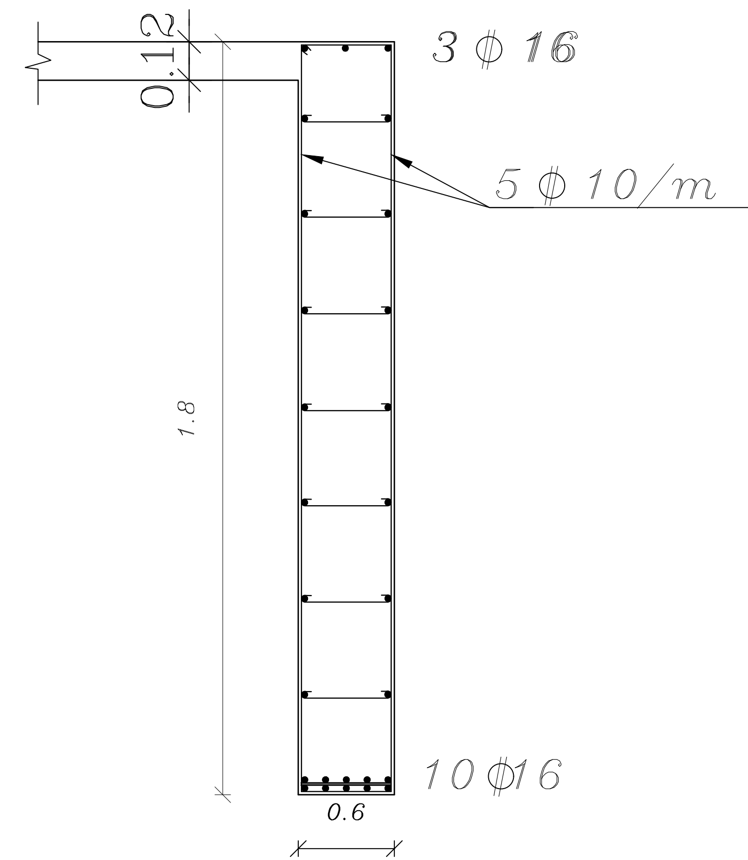
SEC (X-X)
