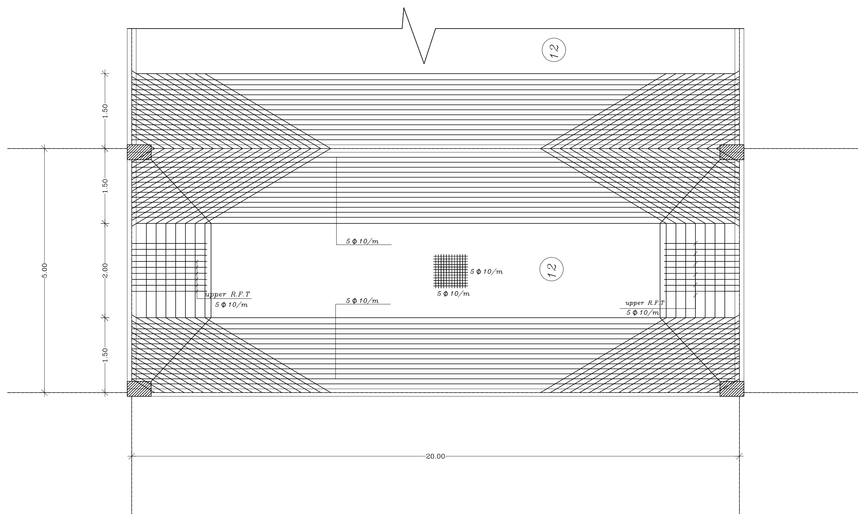
DETAILS OF RFT IN PLAN
