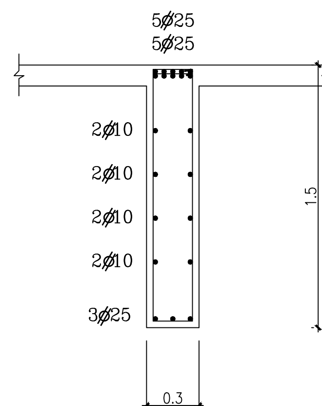
Section 1-1
