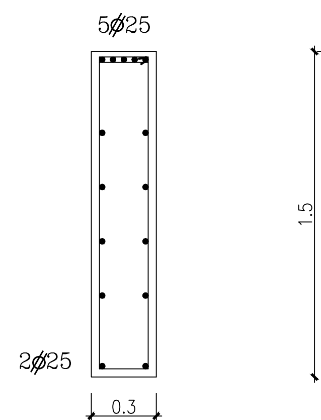
Section 4-4
