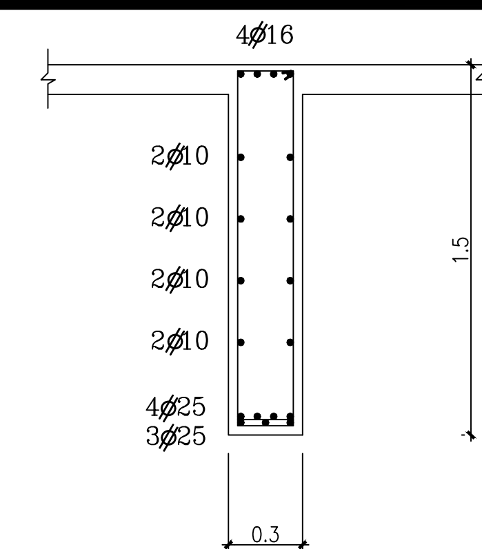
Section 1-1
