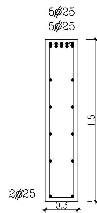
Section 3-3
