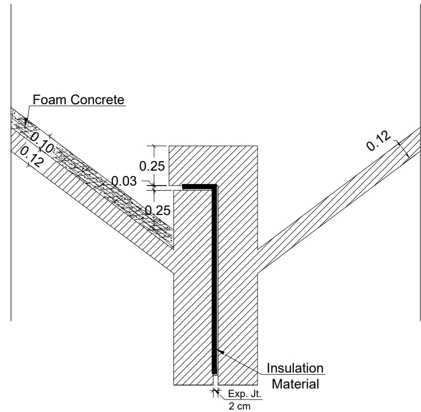
Expansion Joint
