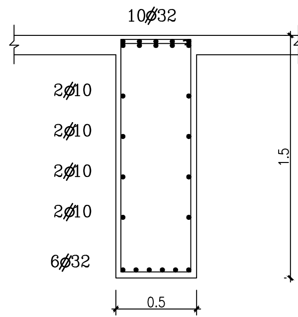
Section 1-1
